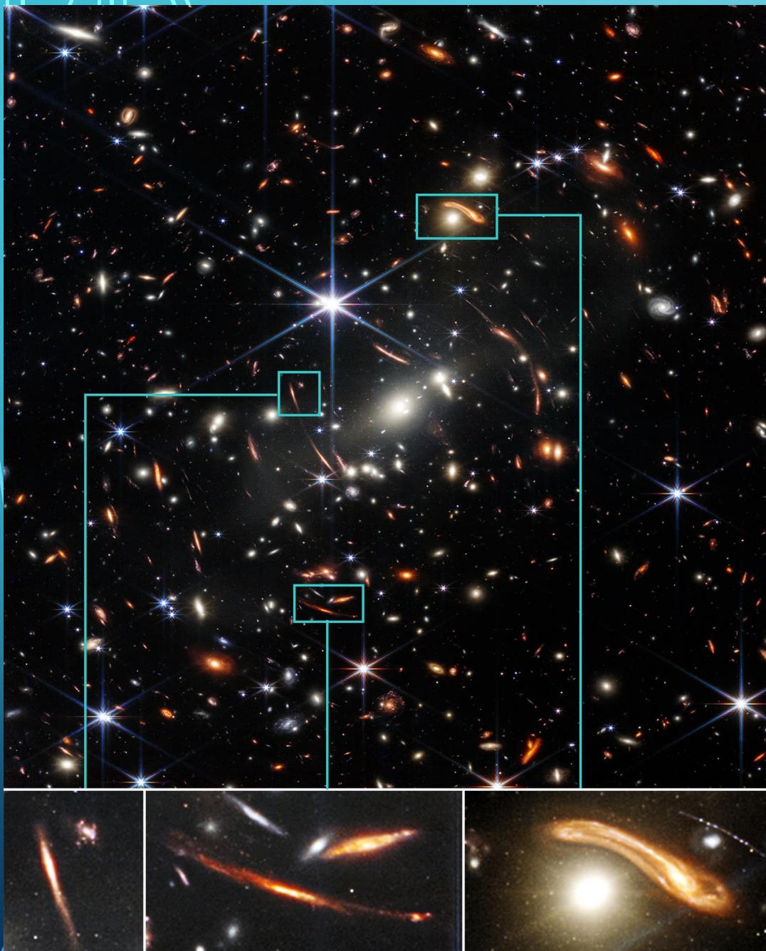
Light from galaxies that has taken many billions of years to reach us
